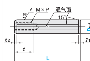
MSTM (带拉拔螺纹m6型)
